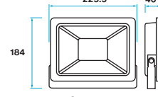
50 watt
